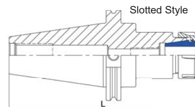
Slotted Style
