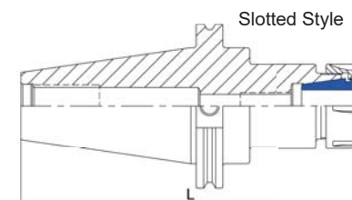
Slotted Style
