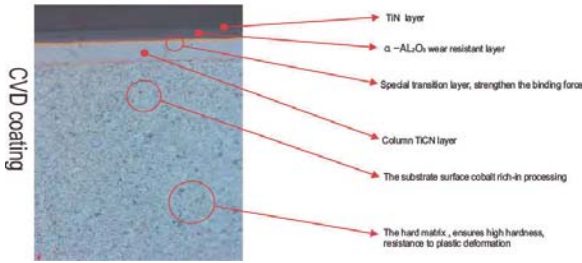
Carbide Insert CVD Coated CCMT32.51 Black/Yellow #2200-1014
